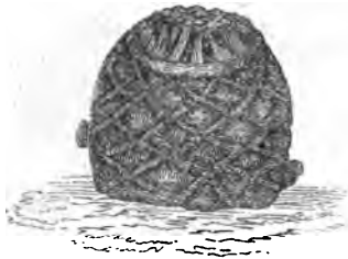
MANTELLIA NIDIFORMIS. (Portland Dirt-bed.)
